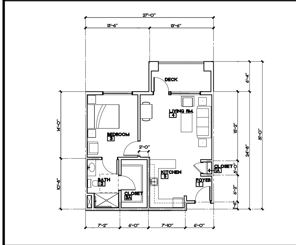
UNIT TYPE - 1.6 AREA: 666.1 S.F. DECK: 85.4 S.F.
