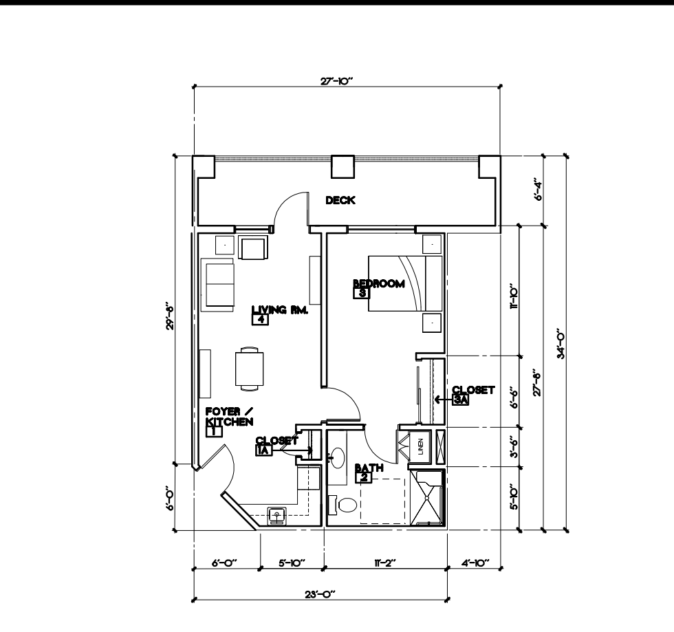
UNIT TYPE - 1.4 AREA: 636.4 S.F. DECK: 170.9 S.F.
