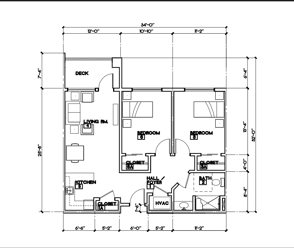
UNIT TYPE - 2.1 AREA: 872.8 S.F. DECK: 76.0 S.F.
