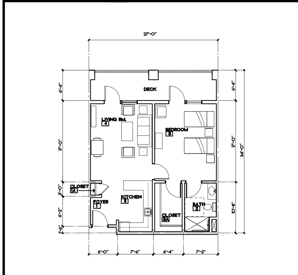
UNIT TYPE - 1.3 AREA: 747.1 S.F. DECK: 170.9 S.F.
