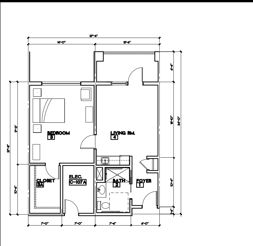
UNIT TYPE - 1.5 AREA: 761 S.F. DECK: 85 S.F.
