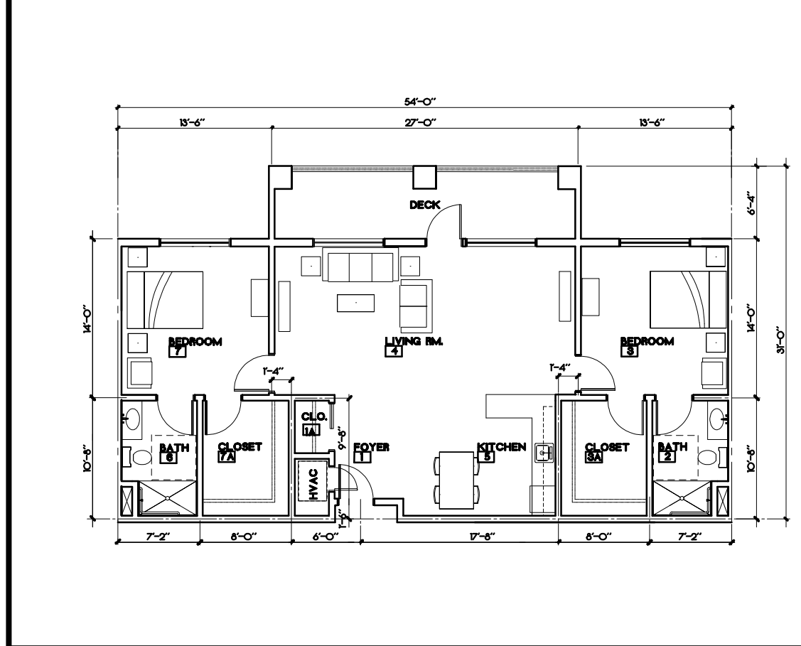
UNIT TYPE - 2.4 AREA: 1332.2 S.F. DECK: 170.9 S.F.
