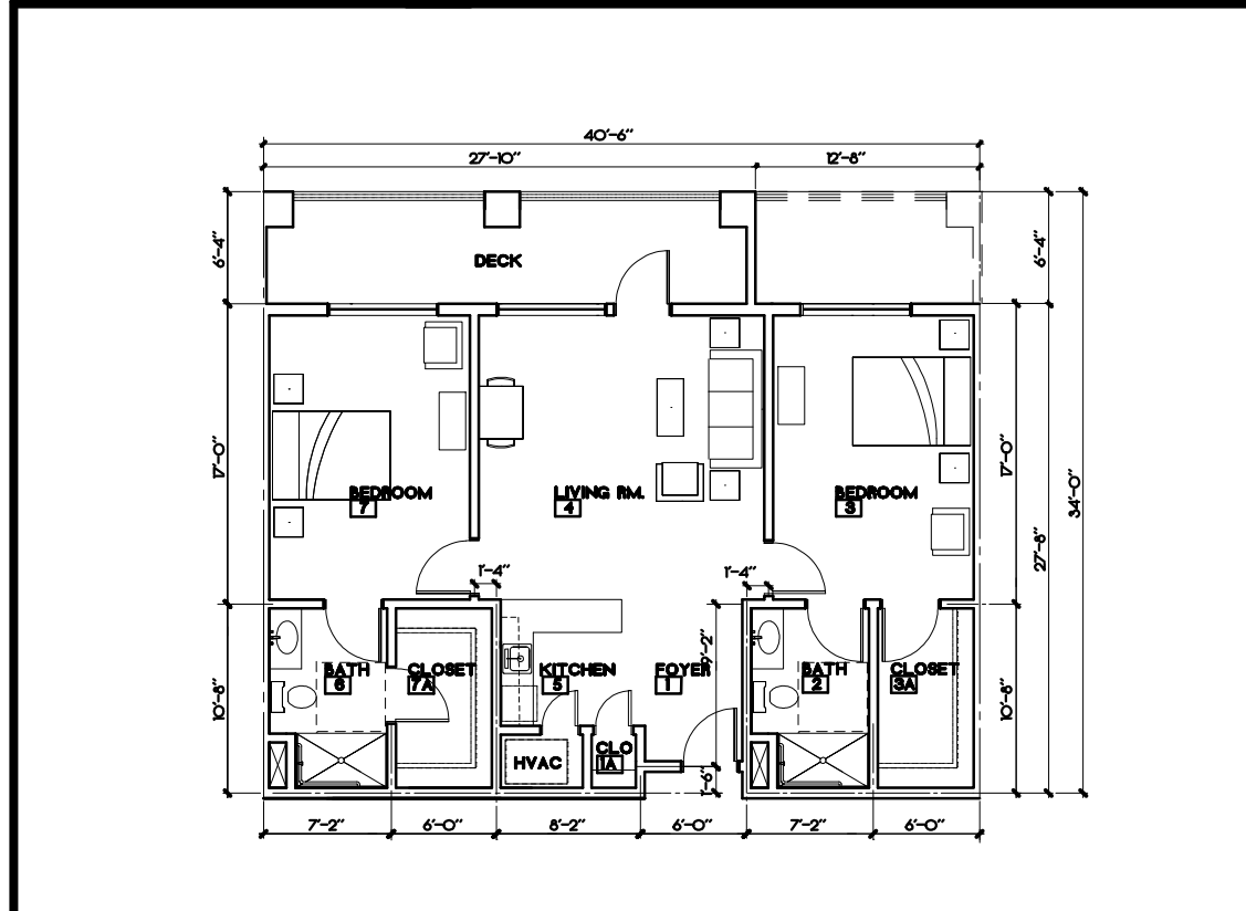
UNIT TYPE - 2.2 AREA: 1120.6 S.F. DECK: 170.9 S.F.
