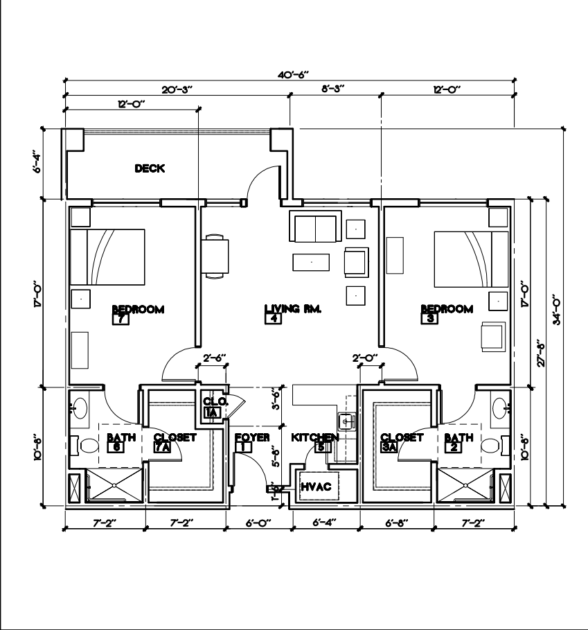
UNIT TYPE - 2.5 AREA: 1120.6 S.F. DECK: 128.2 S.F.
