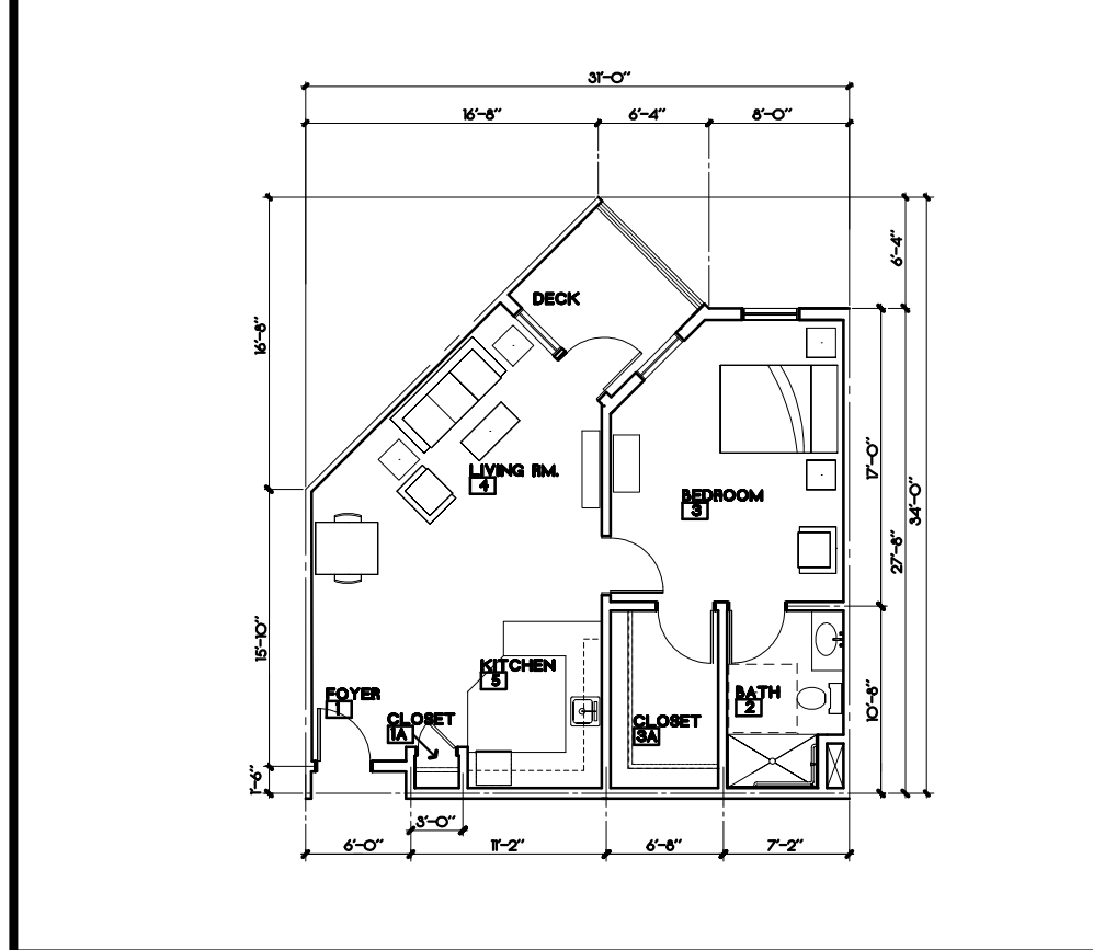
UNIT TYPE - 1.1B AREA: 780.6 S.F. DECK: 63.7 S.F.
