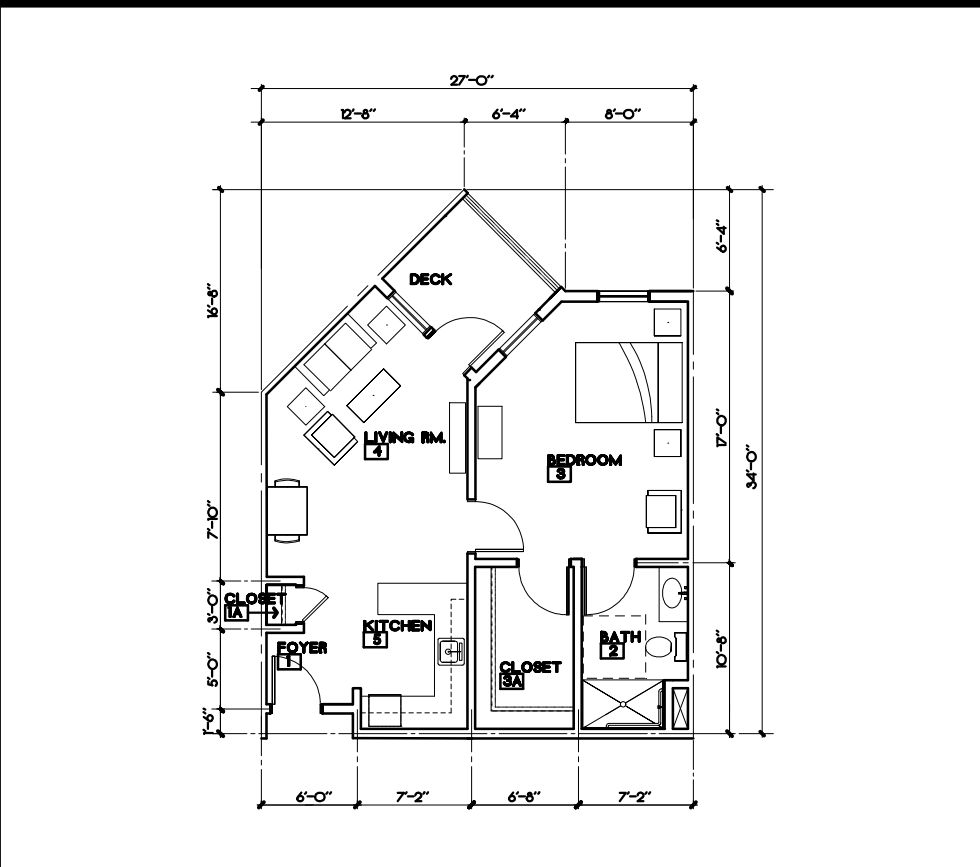
UNIT TYPE - 1.1A AREA: 703.3 S.F. DECK: 63.7 S.F.
