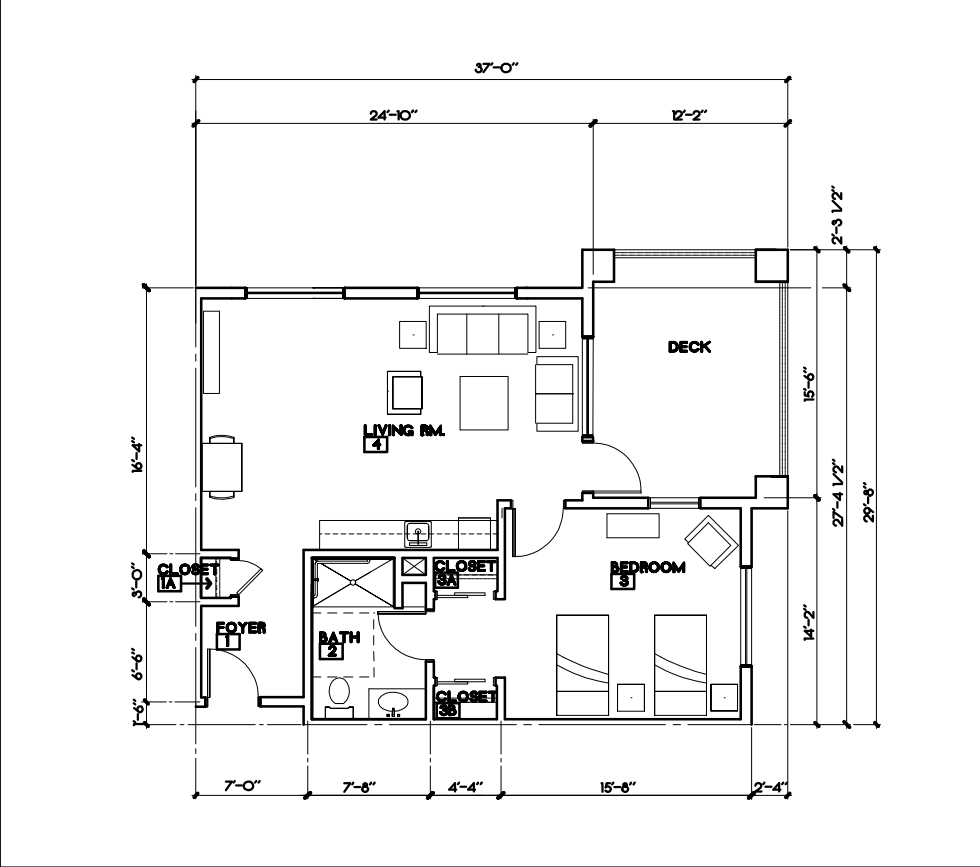
UNIT TYPE - 1.2 AREA: 819.1 S.F. DECK: 188.5 S.F.
