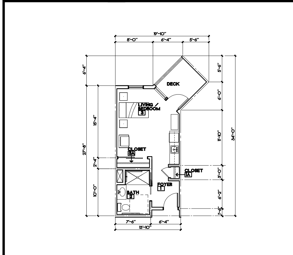
UNIT TYPE - 0.6 AREA: 368.3 S.F. DECK: 63.7 S.F.
