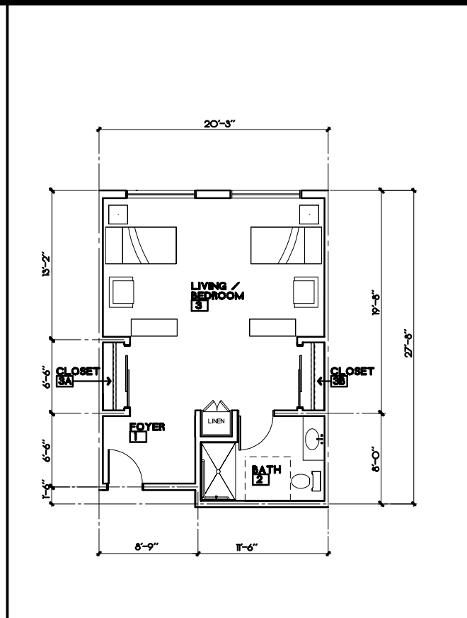
UNIT TYPE - 0.2A (MEMORY SUPPORT) AREA: 560.3
