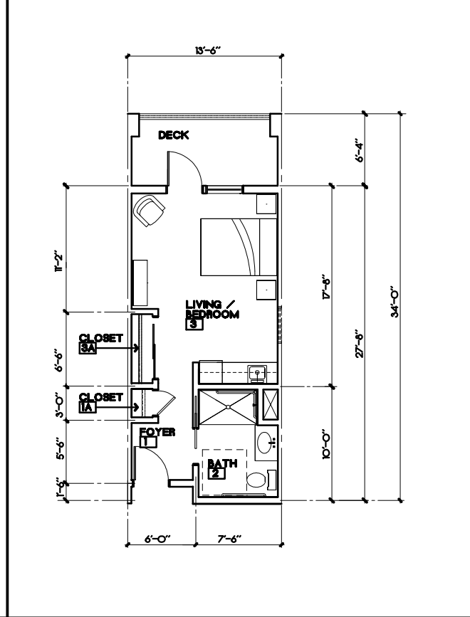
UNIT TYPE - 0.4 (MEMORY SUPPORT) AREA: 373.5 S.F. DECK: 85.4 S.F.
