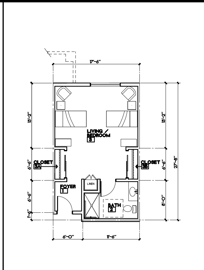
UNIT TYPE - 0.2B (MEMORY SUPPORT) AREA: 484.2 S.F.
