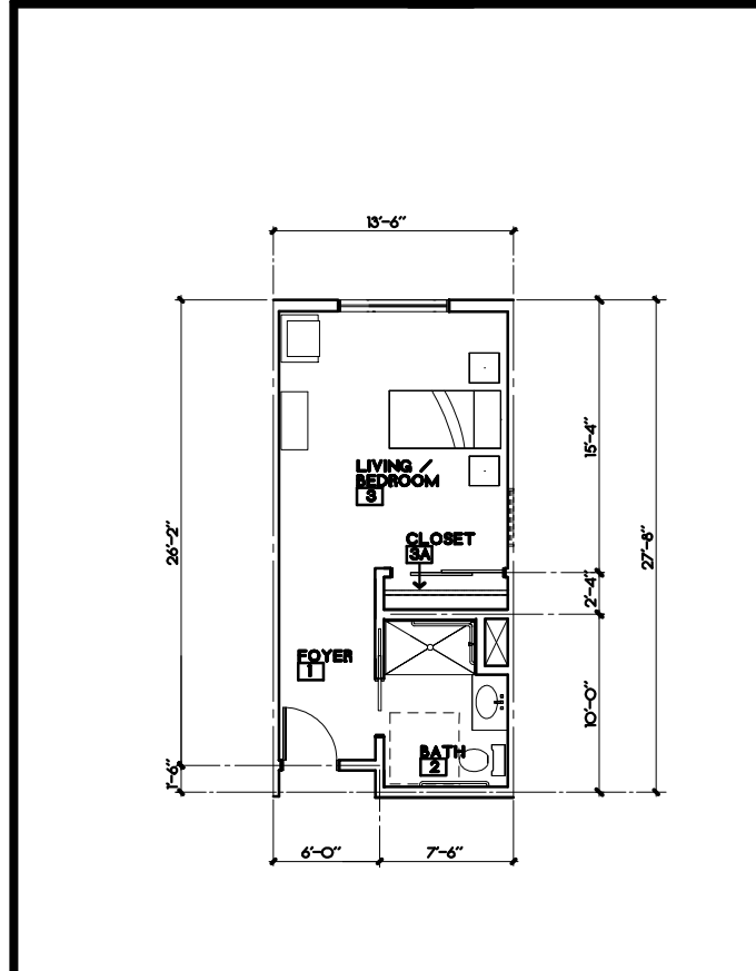
UNIT TYPE - 0.1 (MEMORY SUPPORT) AREA: 373.5 S.F.
