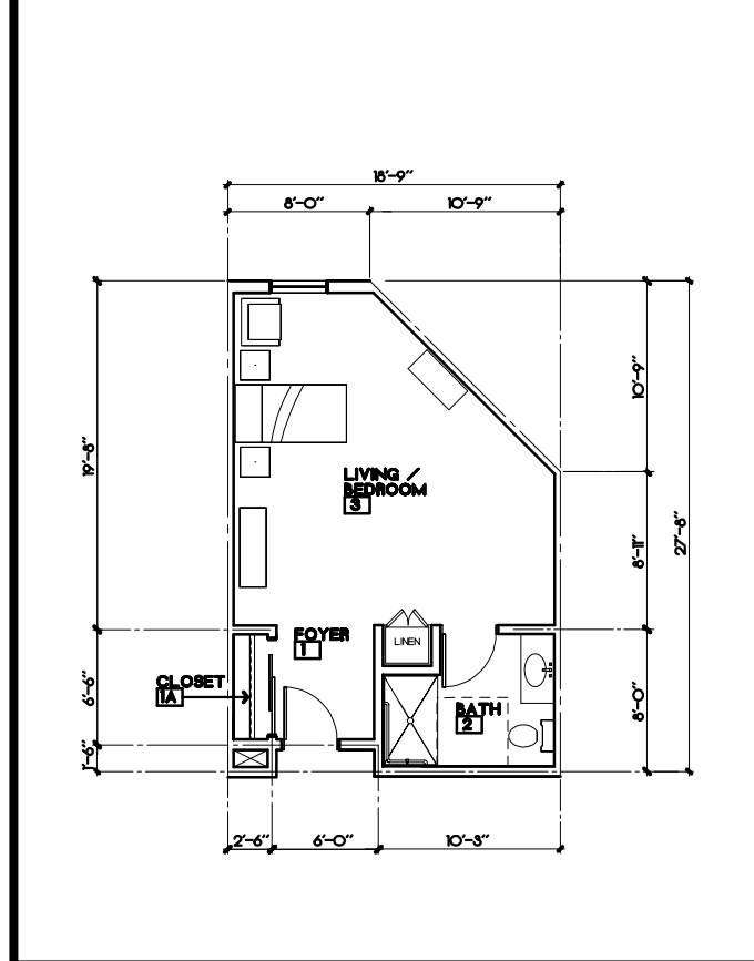
UNIT TYPE - 0.3 (MEMORY SUPPORT) AREA: 461.0 S.F.
