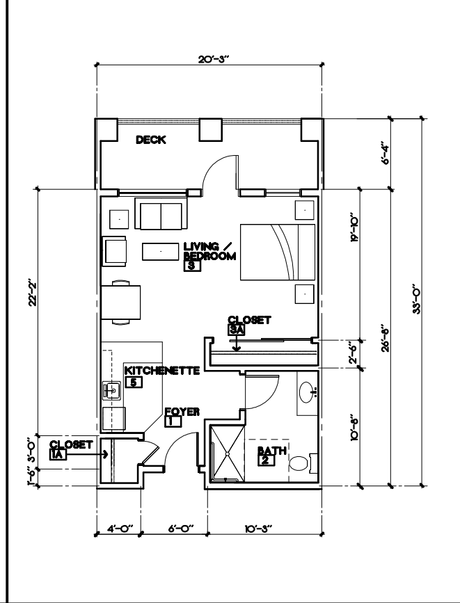
UNIT TYPE - 0.5 (MEMORY SUPPORT) AREA: 560.3 S.F. DECK: 128.2 S.F.
